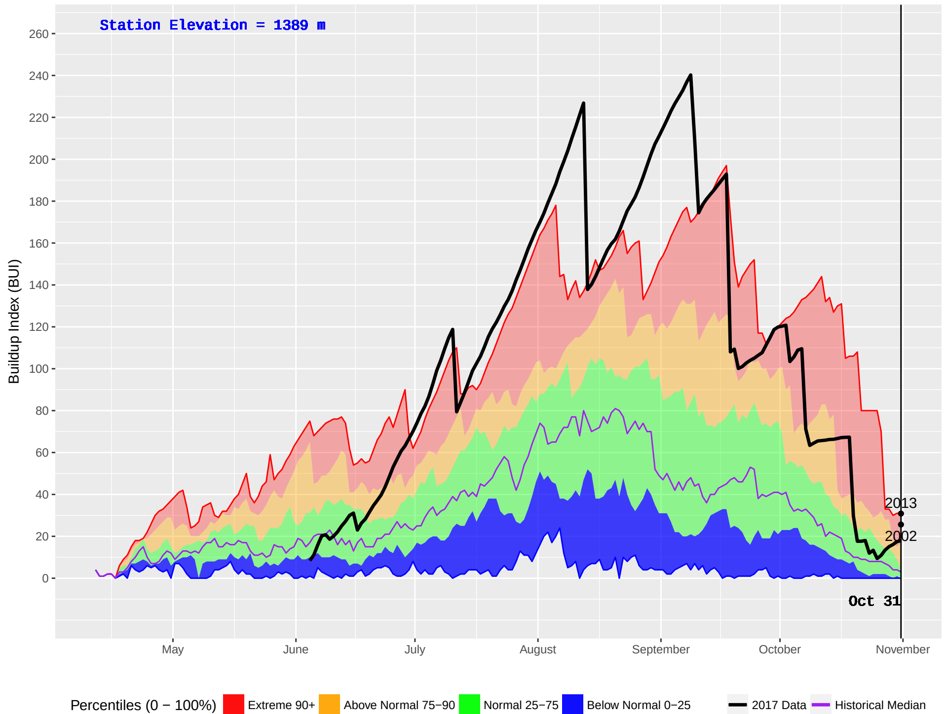
KETTLE 2 (388) : Historical (1987–2016) and Current (2017) Noon Buildup Index (BUI)
