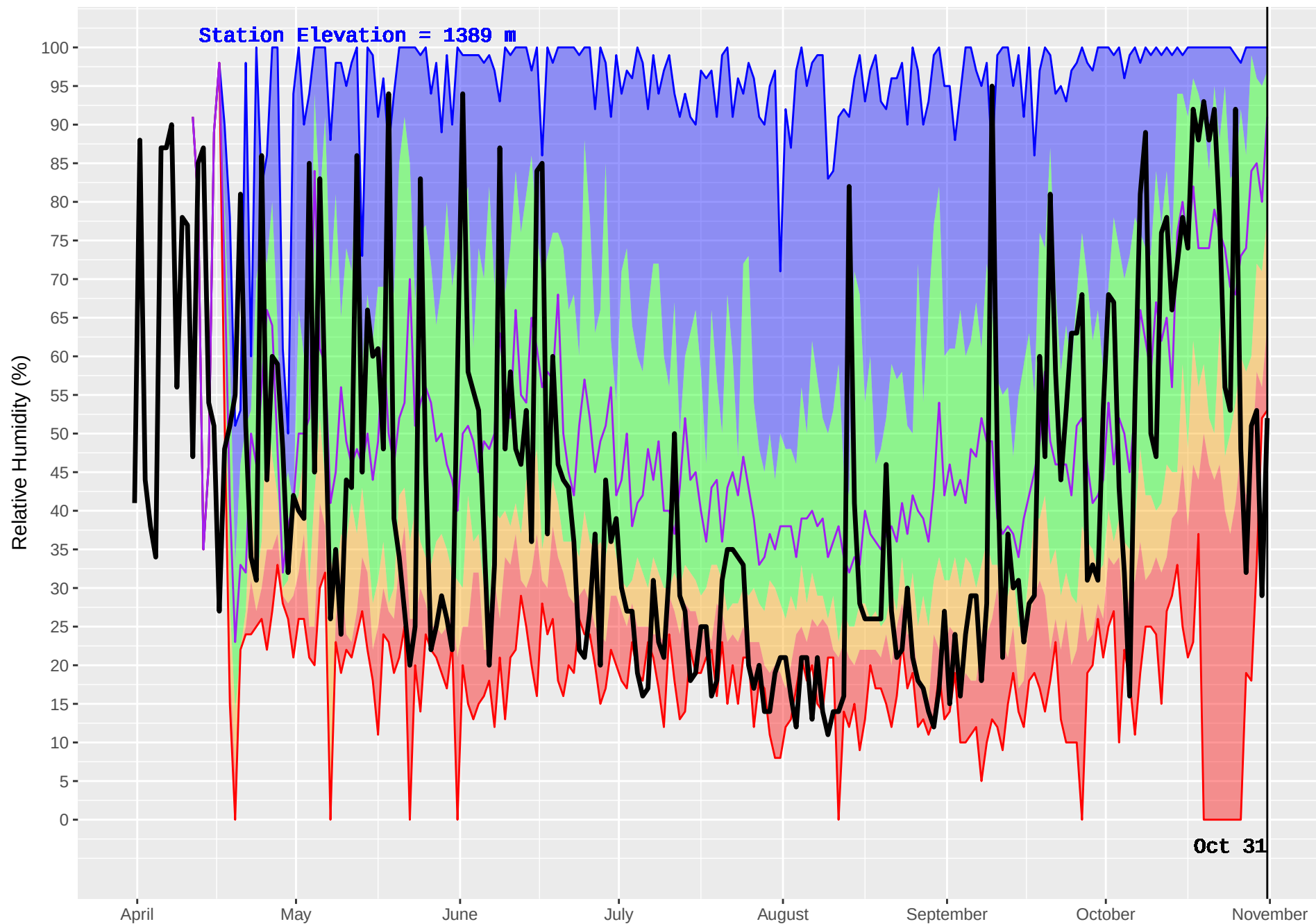
KETTLE 2 (388) : Historical (1987–2016) and Current (2017) Noon Relative Humidity
