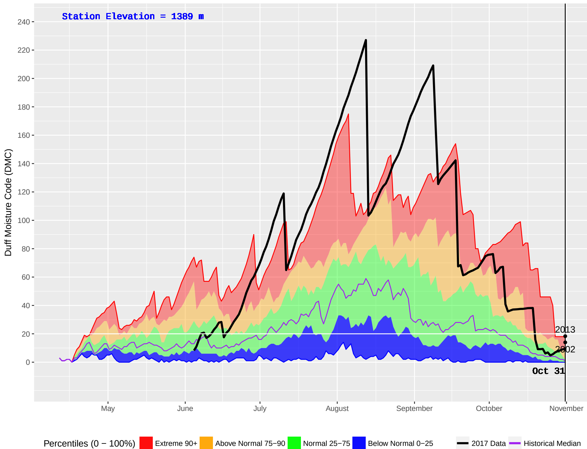
KETTLE 2 (388) : Historical (1987–2016) and Current (2017) Noon Duff Moisture Code (DMC)
