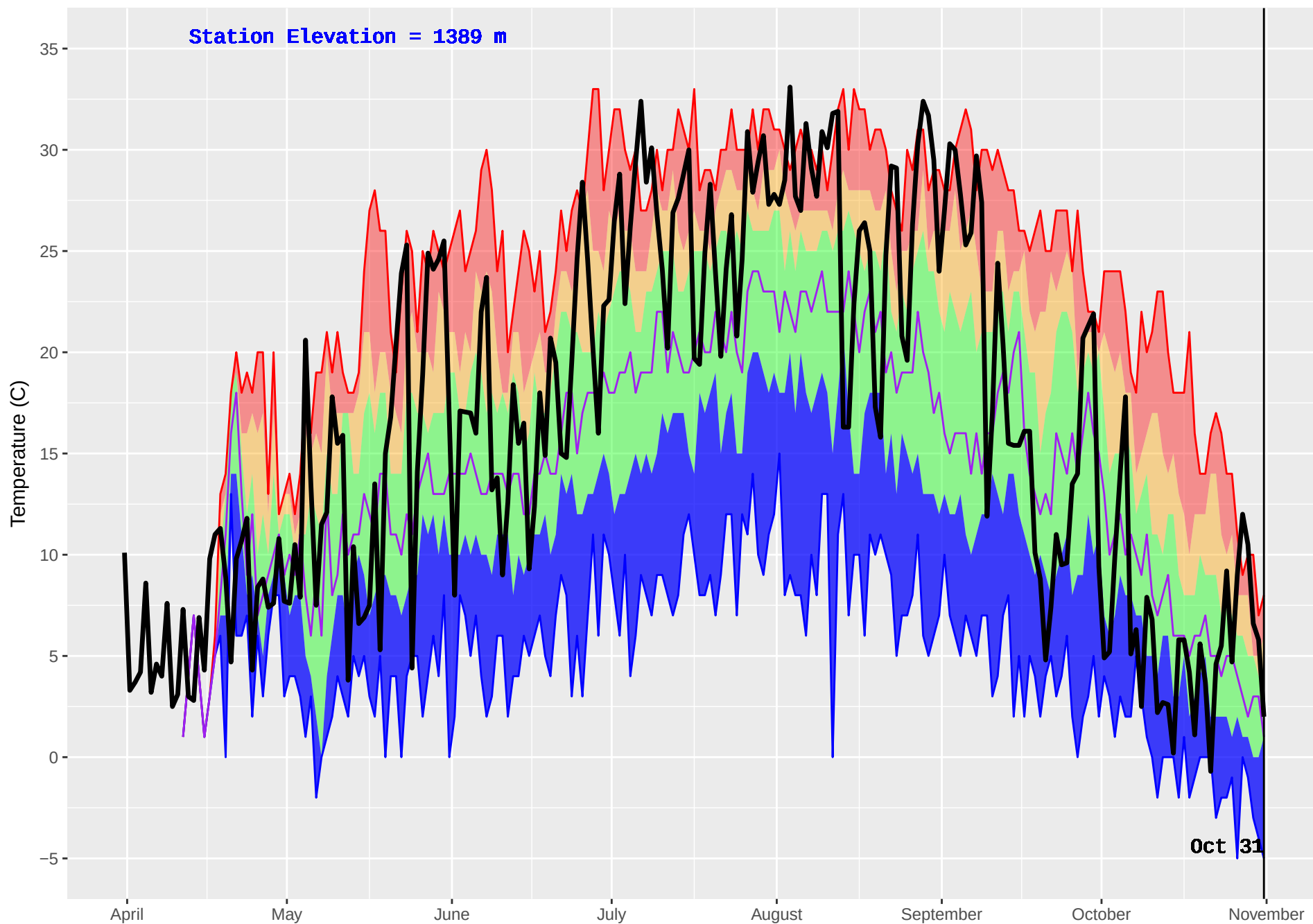
KETTLE 2 (388) : Historical (1987–2016) and Current (2017) Noon Temperature
