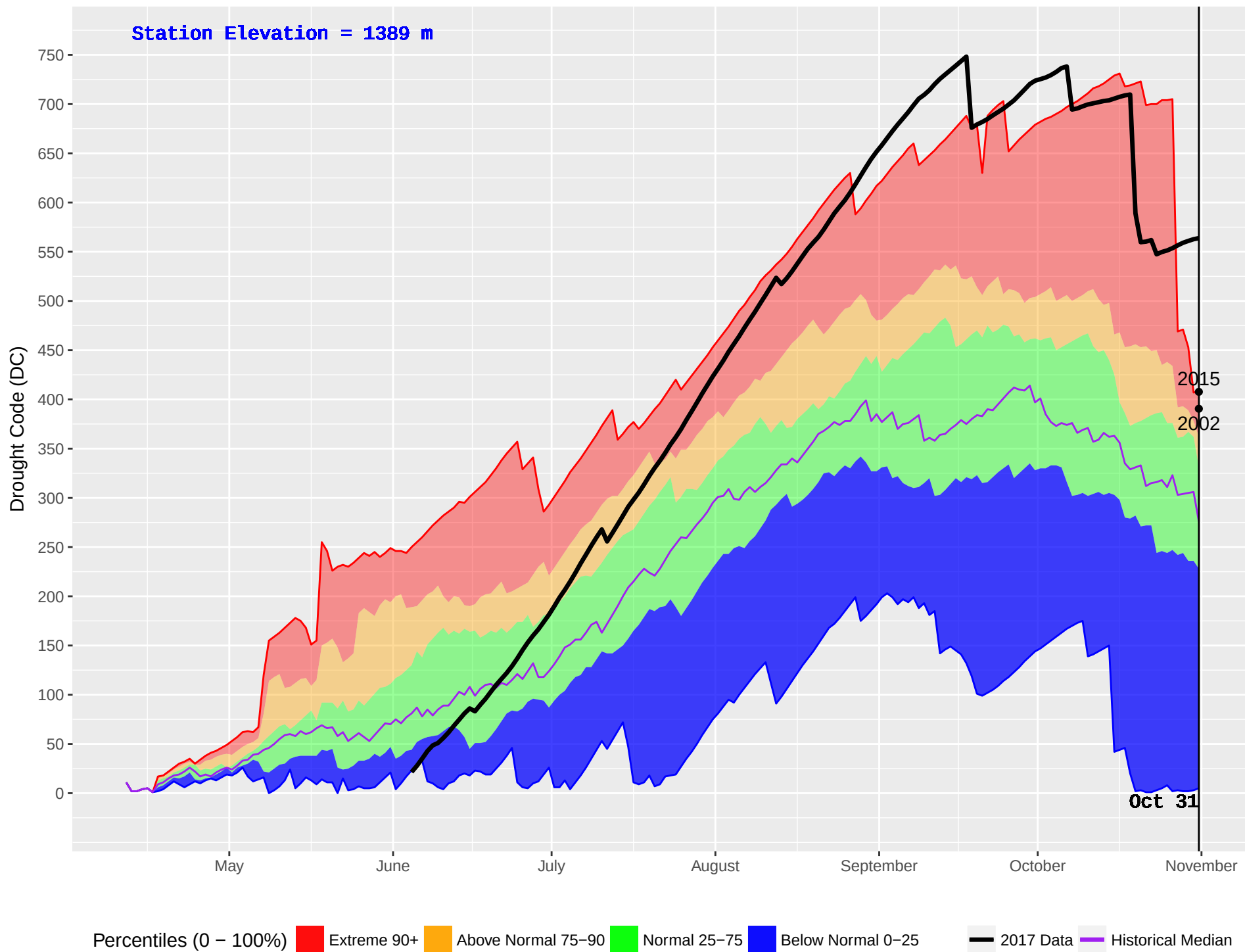
KETTLE 2 (388) : Historical (1987–2016) and Current (2017) Noon Drought Code (DC)
